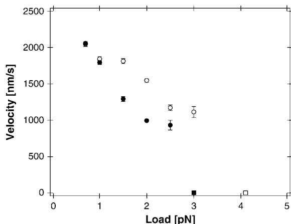
FIGURE 3 NcKin velocities under load. Average velocities v (mean \pm SE) of NcKin reference (open circles, N = 103 - 758 ) and NcKin-SN (solid circles, N = 73 - 512 ) are plotted against applied load. The average velocities of both molecules drop with increasing external forces. Although both molecules display identical average velocities at the lowest tested loads of 0.7 and 1.0 pN, there are apparent differences at higher loads. The rectangles mark the molecules' stall forces where the average velocity is reduced to zero (Fig. 4).
