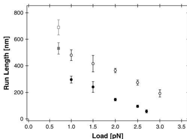
FIGURE 2 NcKin run lengths under load. Average run lengths ( \text{mean} \pm \text{SE} ) of NcKin-wild-type (open circles, N = 50 - 477 ) and NcKin-SN (solid circles, N = 40 - 258 ) versus applied load. All measurements were performed under constant force conditions. The data points at 0.7 pN (gray squares) are likely to present an underestimate due to the limited range of the feedback system. Both molecules display a significantly increasing processivity at loads smaller than 1.0 pN.
